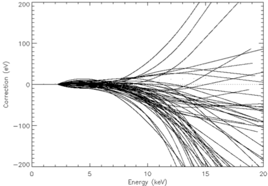
Figure 18. Display of spline offset curves for all 52 operating NICER detectors. The correction is relative to optmv12.
