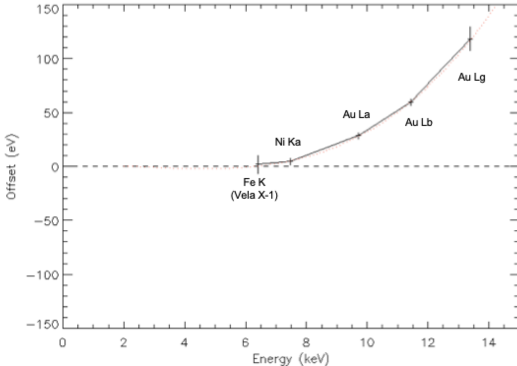
Figure 17. Broad-scale energy offset fit to line centroids, with spline fit (red dotted line), again for DET_ID=00. The offset is relative to optmv12.
