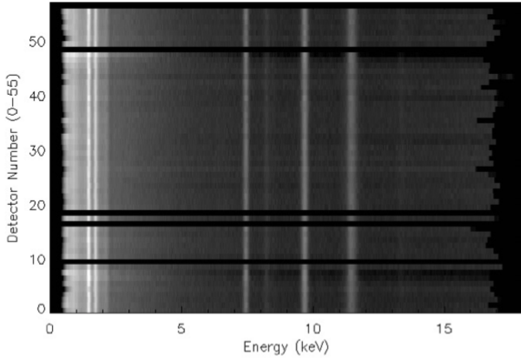
Figure 19. Per detector NICER SAA spectra (ame as Figure 15) but with energy scale optmv13.
