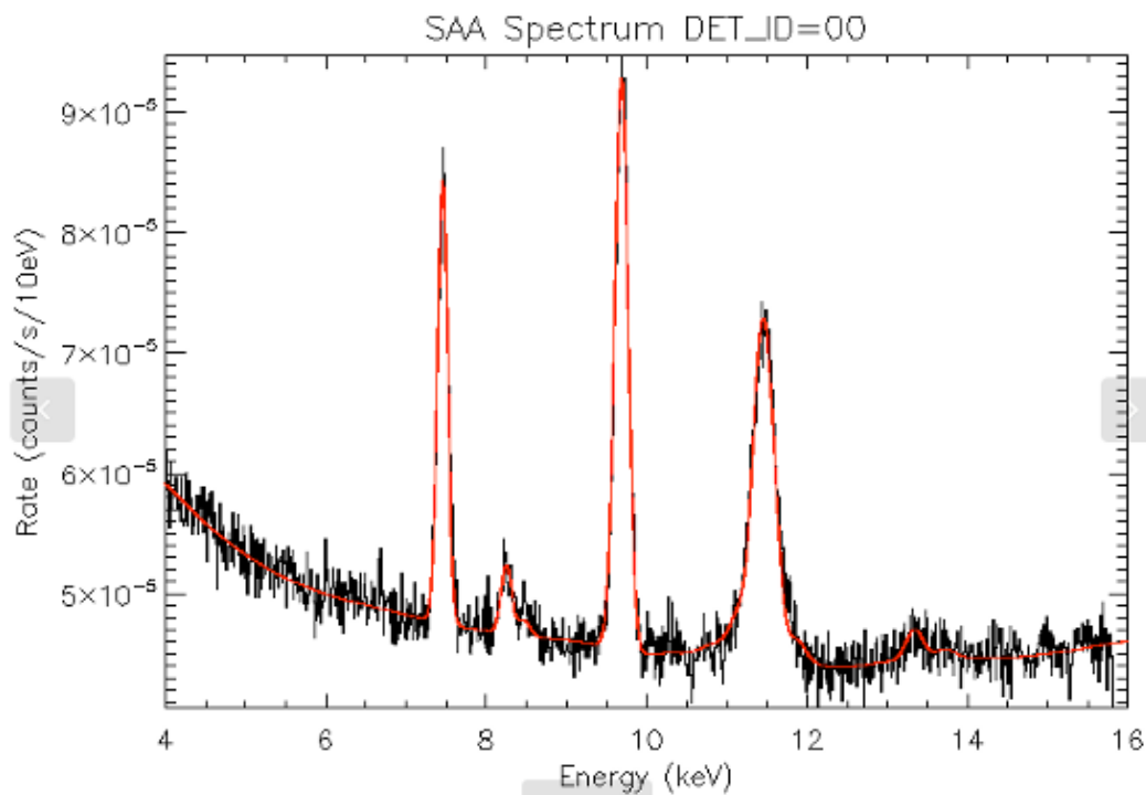
Figure 16. Example per-detector NICER SAA spectrum (black) and line+spline fit (red) for DET_ID=00.
