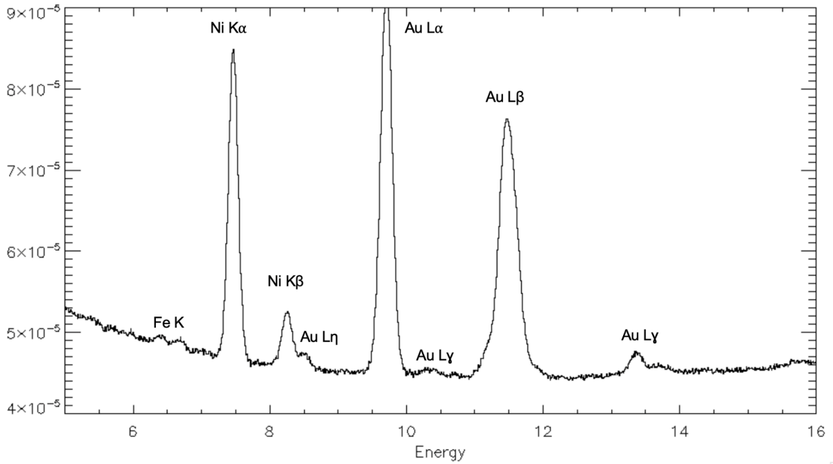
Figure 14. Updated NICER fluorescent line spectrum (compare to Figure 10) during SAA passages, with complexes labeled.
