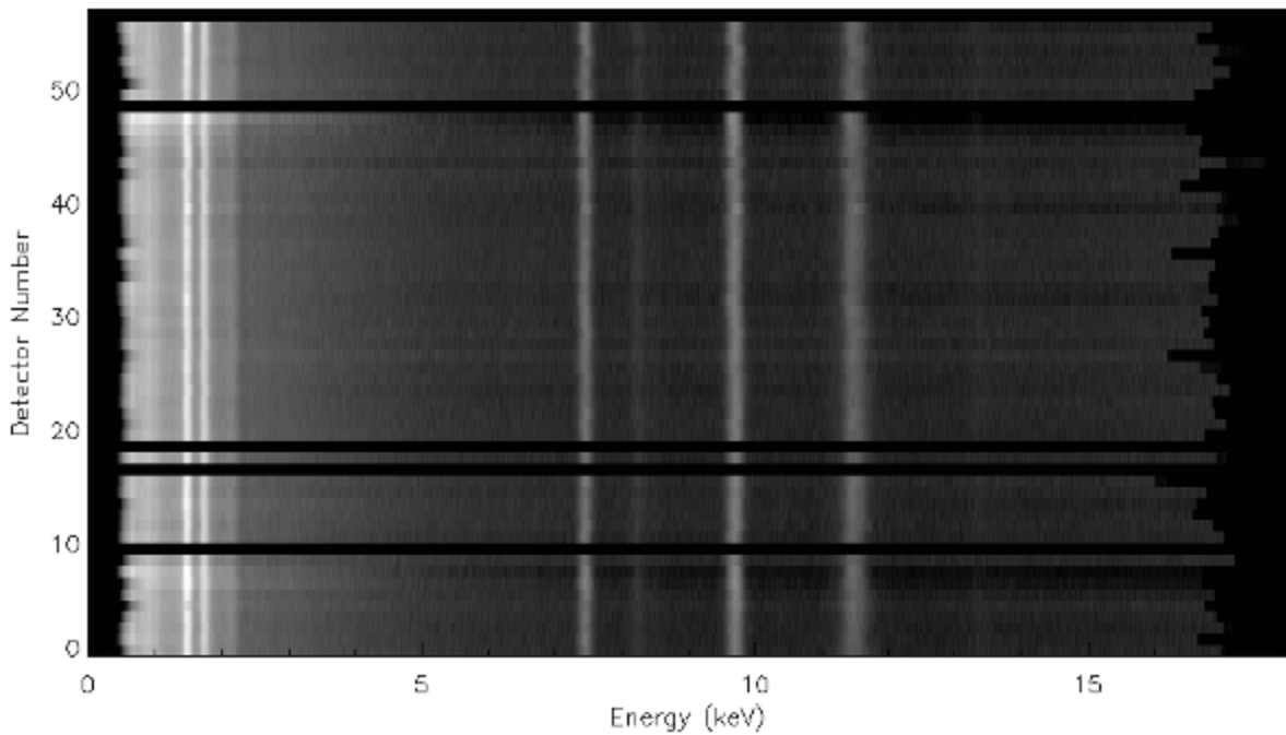
Figure 15. Per-detector spectra NICER SAA data using optmv12 energy scale solution.
