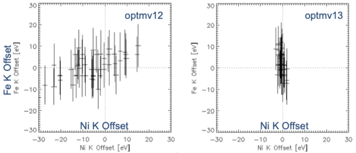
Figure 20. Comparison of Ni K and Fe K offsets using optmv12 (left) and optmv13 (right).
