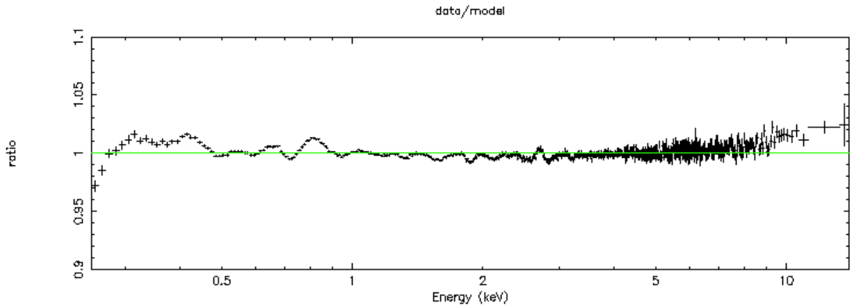
Figure 2. Residuals after using calibration release xti20221001 with the Crab Nebula (no change since previous release)
