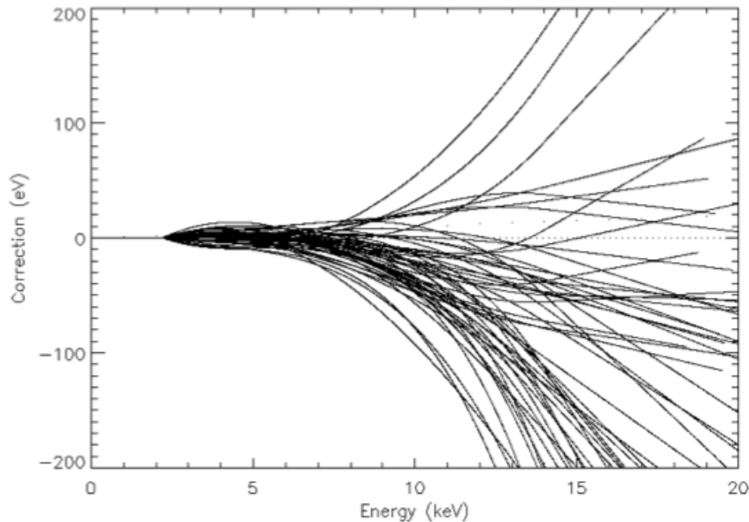
Figure 3. Change to slow channel energy scale due to new optmv13 solution.
