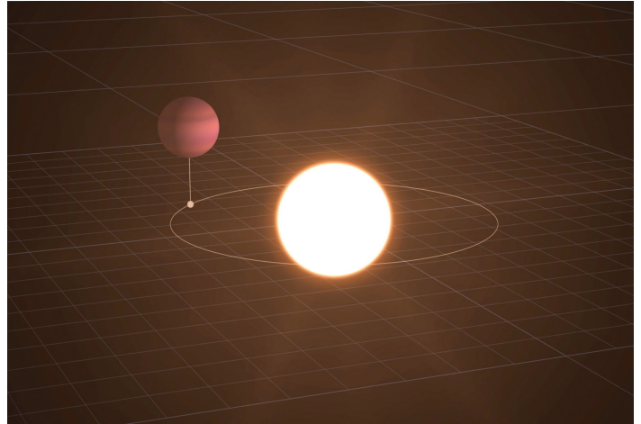
Artist impressions of how the WD 1856 system may have evolved. Image credits: NASA/JPL-Caltech/ NASA’s Goddard Space Flight Center
