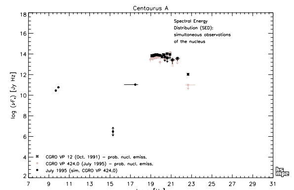
Fig. 6: Simultaneous observations of the nucleus (Only simultaneous observations involving more than one instrument are included)
