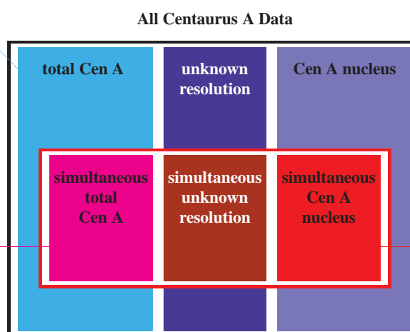
Fig. 5: Classification of observations
