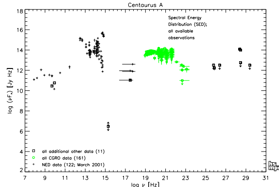
Fig. 2: All available Cen A observations
