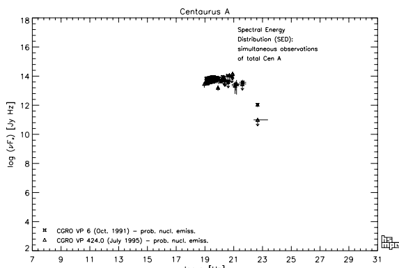
Fig. 4: Simultaneous observations of the unresolved galaxy (Only simultaneous observations involving more than one instrument are included)
