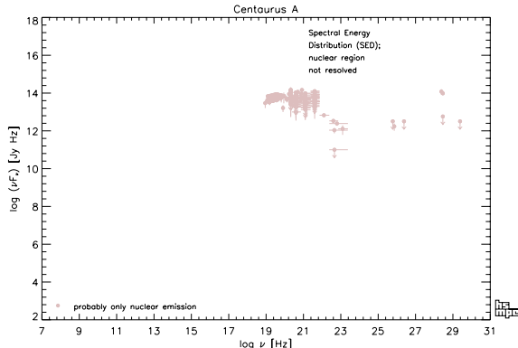
Fig. 1: Total Cen A region (nucleus not resolved)
