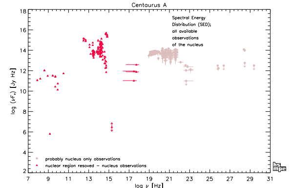
Fig. 3: Observations of the Cen A nucleus
